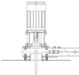
Spring-suspended lid
