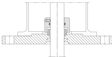
Labyrinth seal
