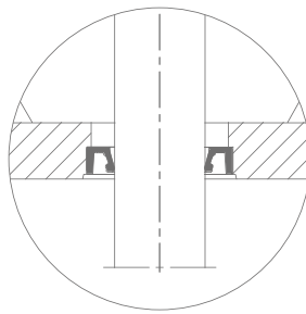
Radial shaft seal ring
