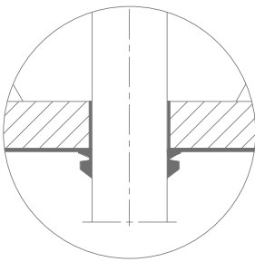
V-ring lip seal
