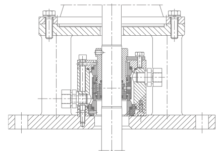
Mechanical seal (single- or double-acting)
