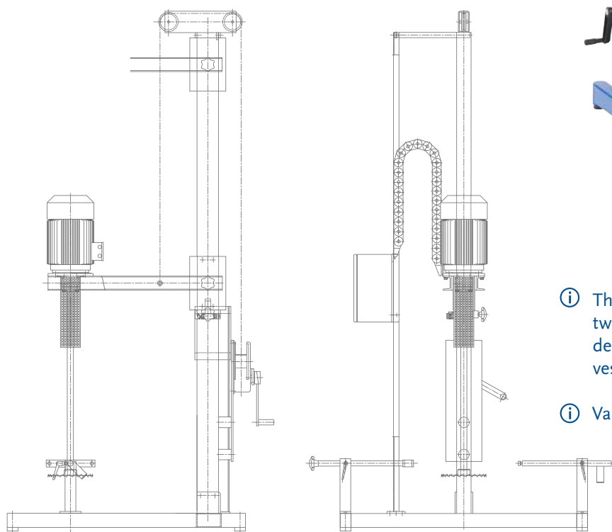
Side and front view of a SRW
