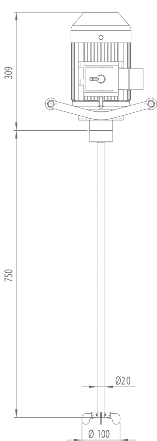
FR with one folding propeller
